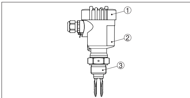
Fig. 1: VEGASWING 61
