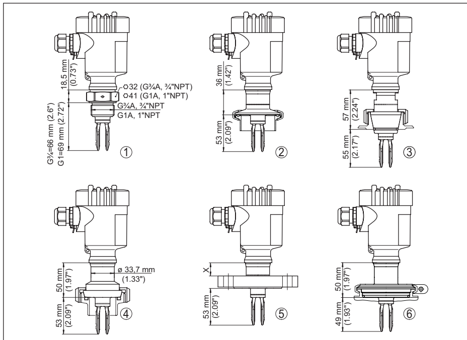
Fig. 20: VEGASWING 61
