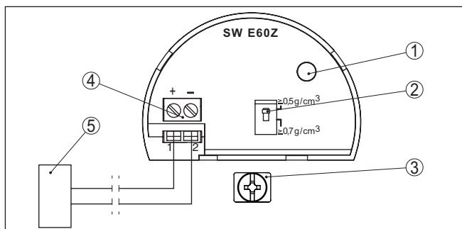
Fig. 8: Electronics and connection compartment
