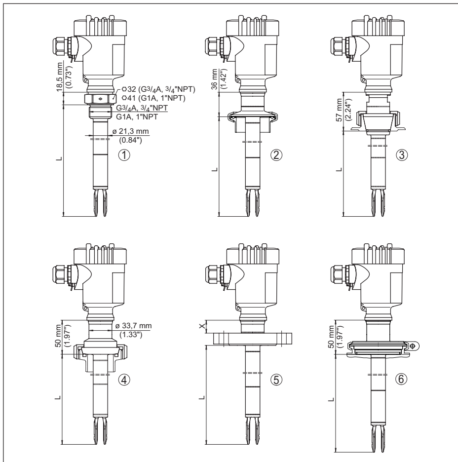
Fig. 20: VEGASWING 63
