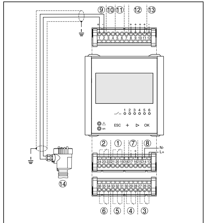
Fig. 14: Wiring plan for two-wire sensor
