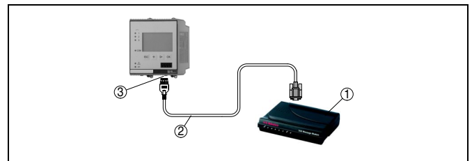
Fig. 25: Connection of the modem via RS232
