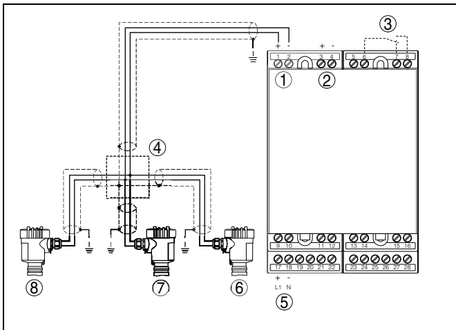
Fig. 17: Wiring plan for two-wire sensors
