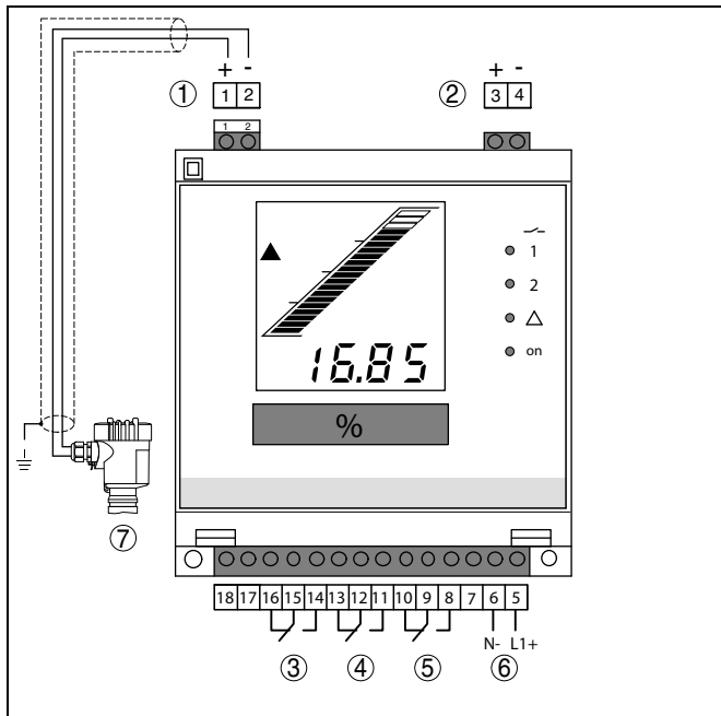
Fig. 13: Wiring plan for two-wire sensor
