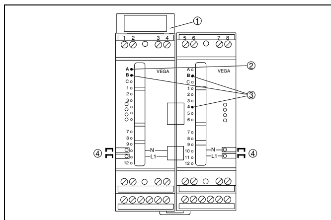
Fig. 10: Plug-in socket VEGAMET
