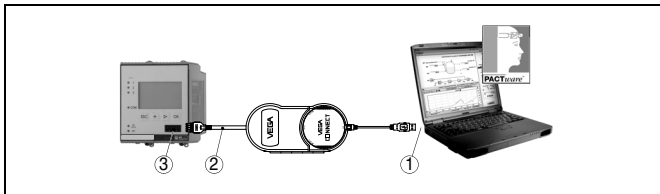
Fig. 22: Connection via VEGACONNECT
