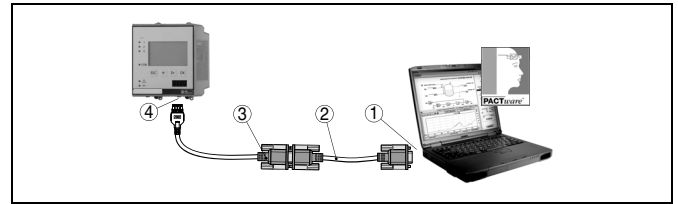
Fig. 24: Connection of the PC via RS232
