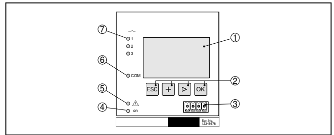
Fig. 20: Indicating and adjustment elements
