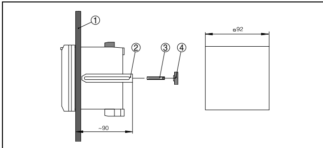
Fig. 4: Front panel mounting
