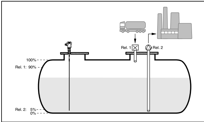
Fig. 2: Example for a level measurement, cylindrical tank
