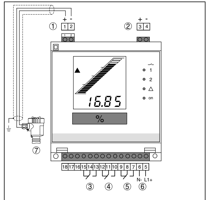
Fig. 12: Wiring plan for two-wire sensor
