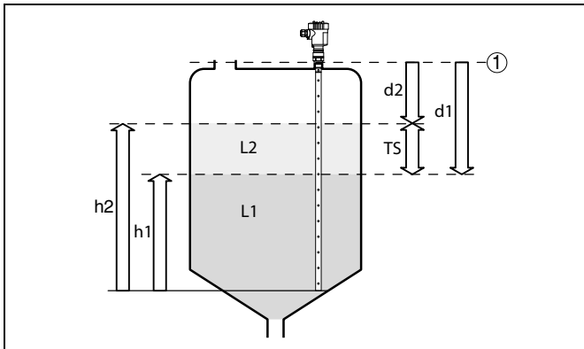
Fig. 3: Interface measurement
