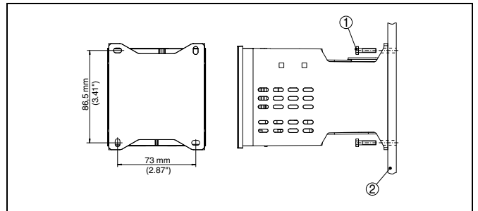
Fig. 8: Screw mounting
