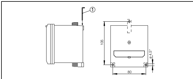
Fig. 5: Screw mounting
