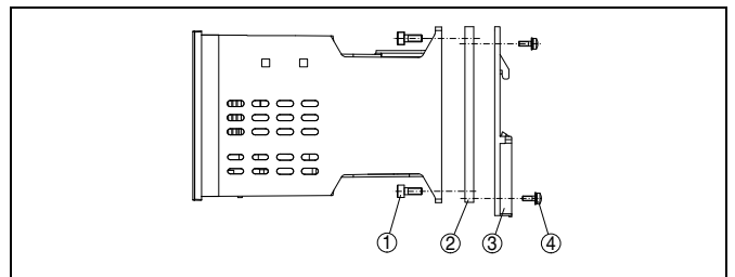
Fig. 9: Carrier rail mounting
