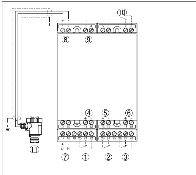
Fig. 15: Wiring plan for two-wire sensor
