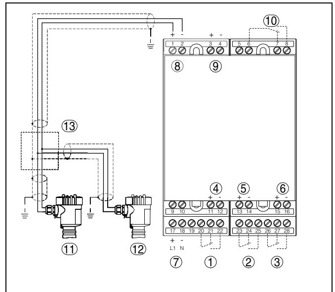
Fig. 16: Wiring plan for two-wire sensors
