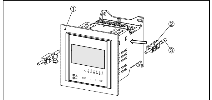
Fig. 7: Front panel mounting
