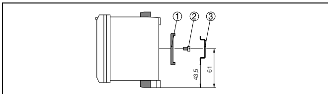
Fig. 6: Carrier rail mounting
