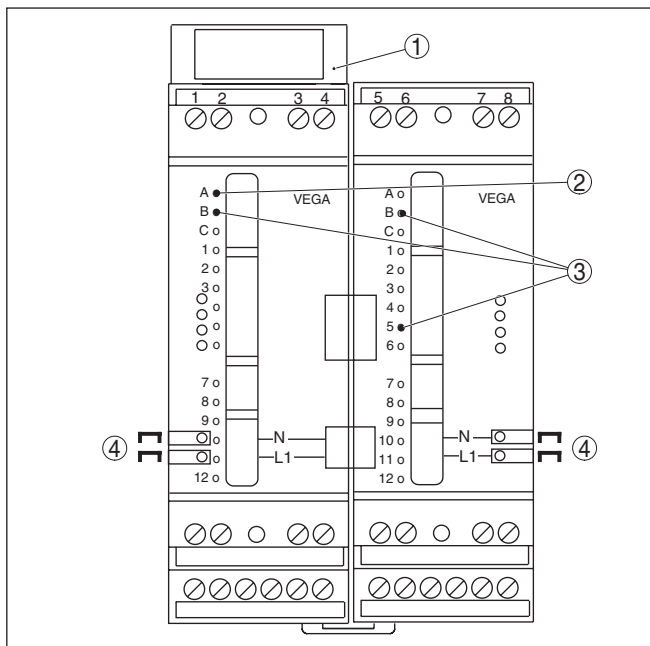
Fig. 2: Klemsokkel VEGASCAN 693
