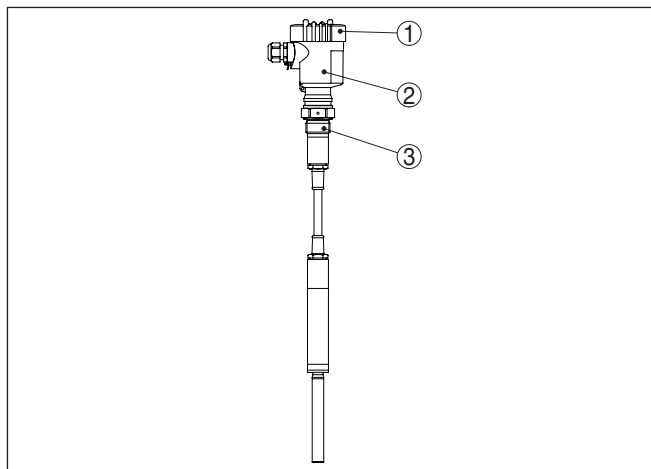
插图. 1: VEGAVIB 62, 带塑料外壳
