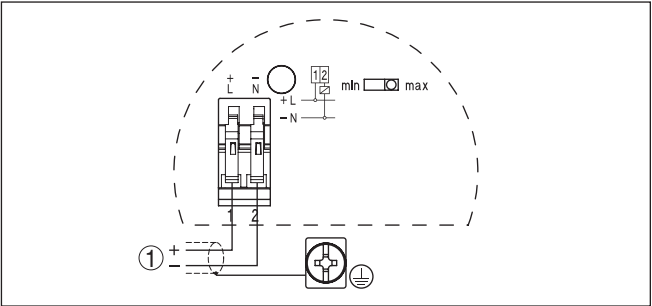
Fig. 9: Wiring plan 1 Shielding
