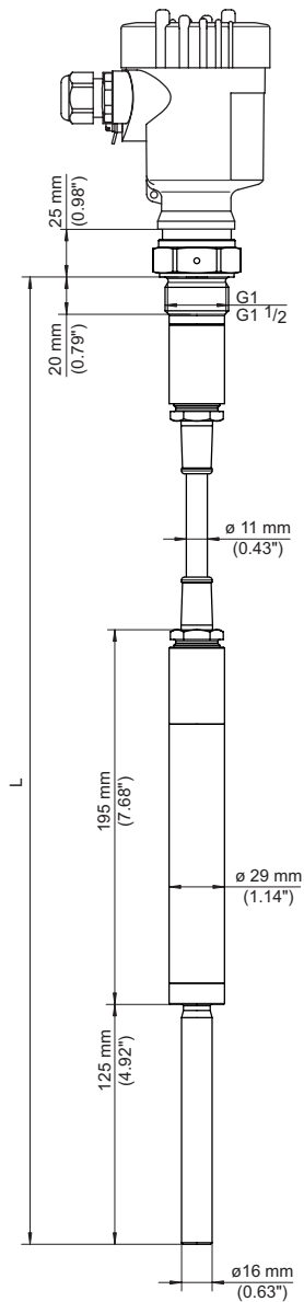
Fig. 13: VEGAVIB 62 with PUR suspension cable
