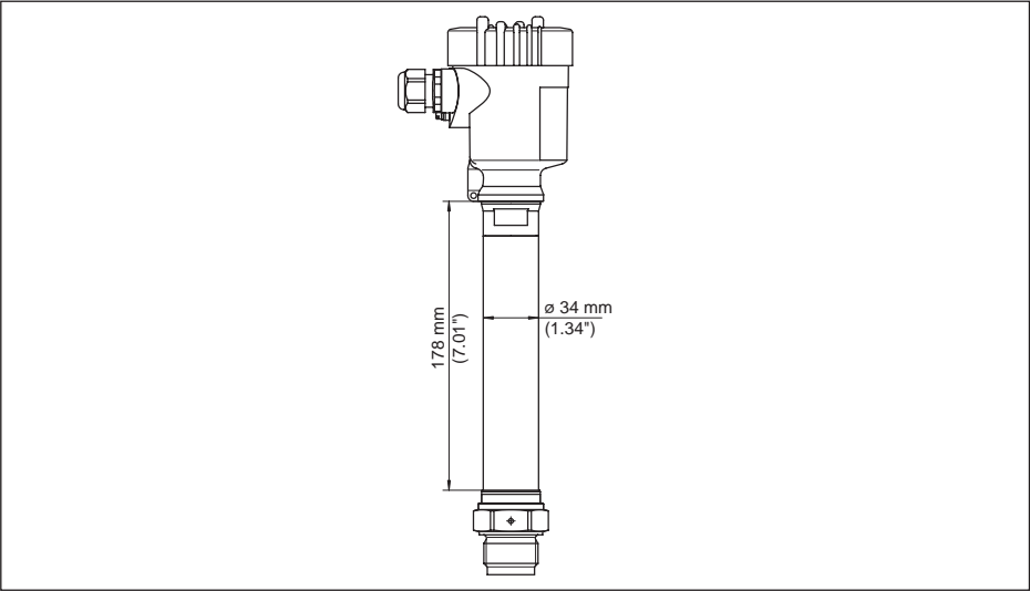
Fig. 31: Temperature adapter
