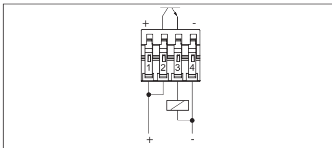
Fig. 11: PNP action
