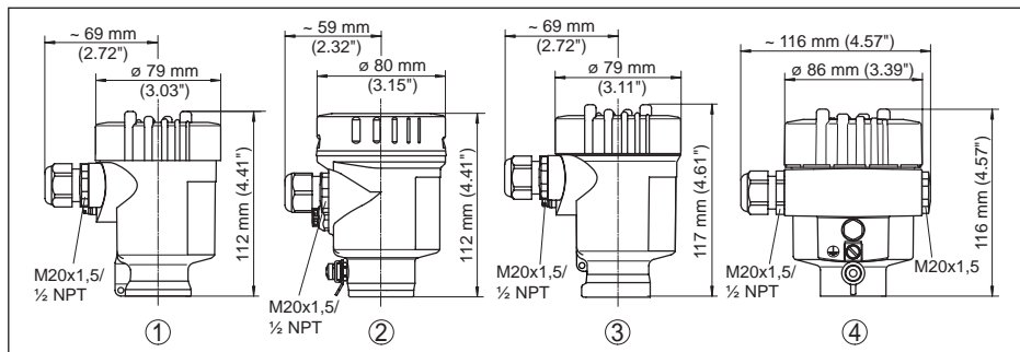
Fig. 27: Housing versions in protection IP 66/IP 67 and IP 66/IP 68; 0.2 bar
