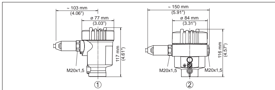
Fig. 28: Housing versions with protection rating IP 66/IP 68 (1 bar)
