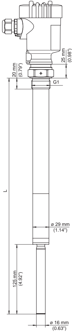
Fig. 29: VEGA VIB 63, threaded version G1 (DIN ISO 228/1)
