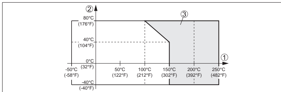
Fig. 26: Ambient temperature - Process temperature
