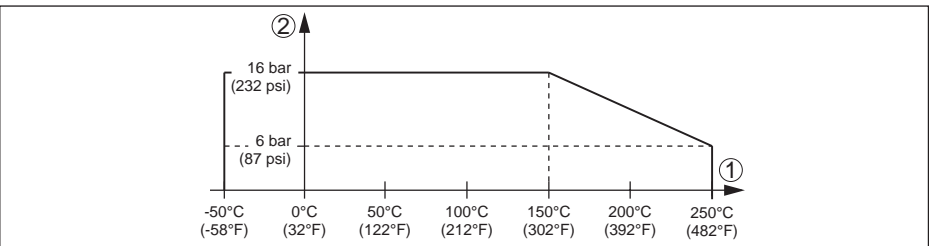
Fig. 25: Process pressure - Process temperature
