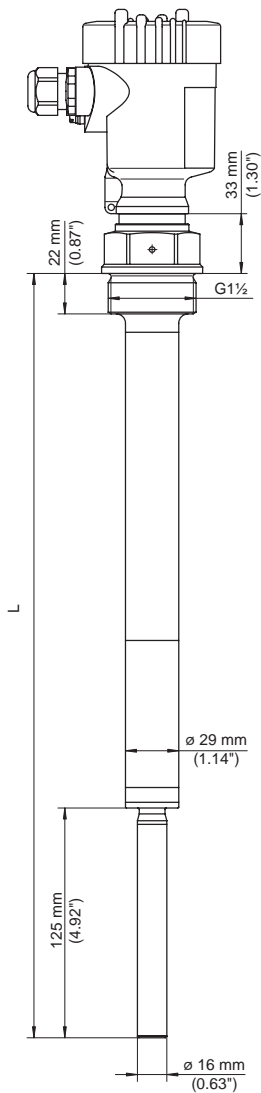
Fig. 30: VEGAVIB 63, threaded version G1½ (DIN ISO 228/1)
