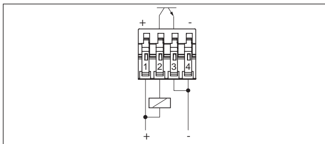
Fig. 10: NPN action
