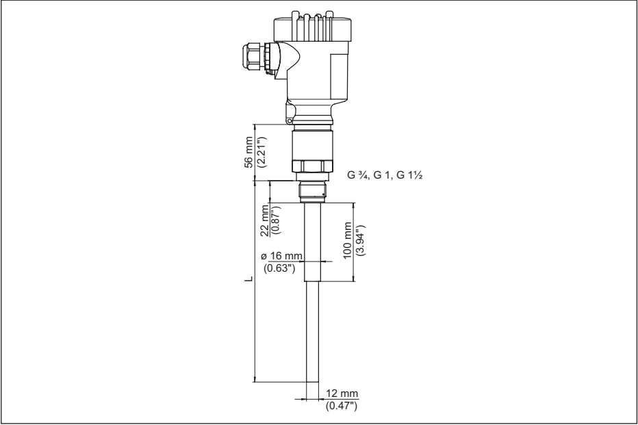
Res. 20: VEGACAP 62, G1 dişli modeli (ISO 228 T1)
