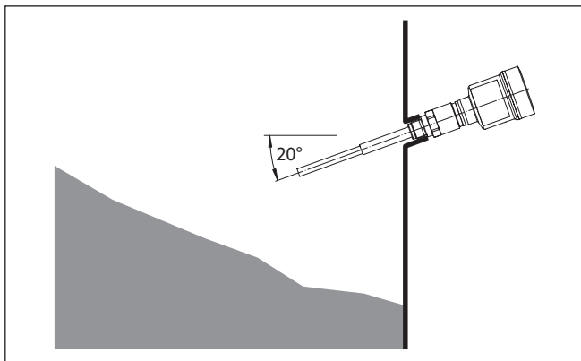
Fig. 6: Montage horizontal
