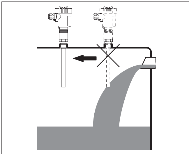
Fig. 5: Instromend medium
