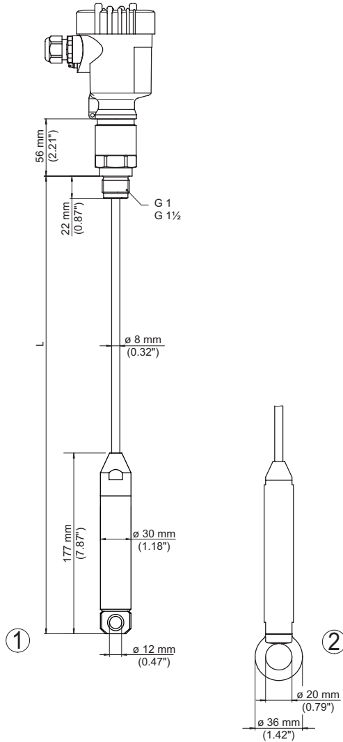
Res. 18: VEGACAP 66, G1 dişli modeli (ISO 228 T1)
