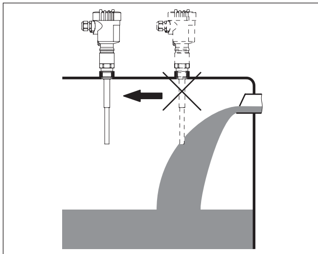
Fig. 7: Instromend medium
