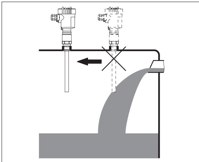
Fig. 7: Instromend medium
