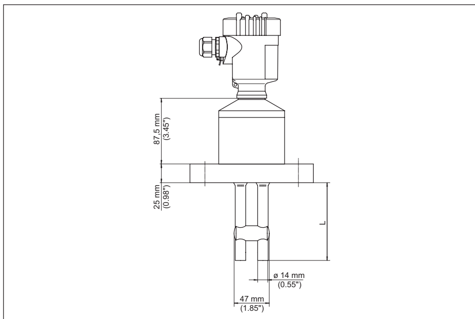
Abb. 34: VEGACAL 69
