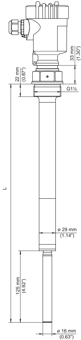
Fig. 35: VEGAVIB 63, threaded version G1½ (DIN ISO 228/1)
