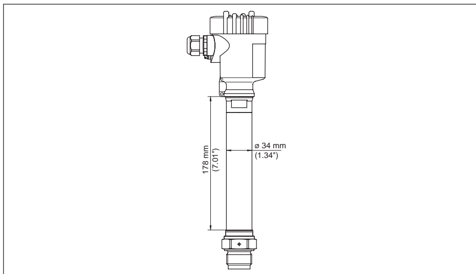
Fig. 36: Temperature adapter
