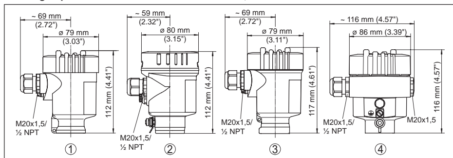
Fig. 32: Housing versions in protection IP 66/IP 67 and IP 66/IP 68; 0.2 bar
