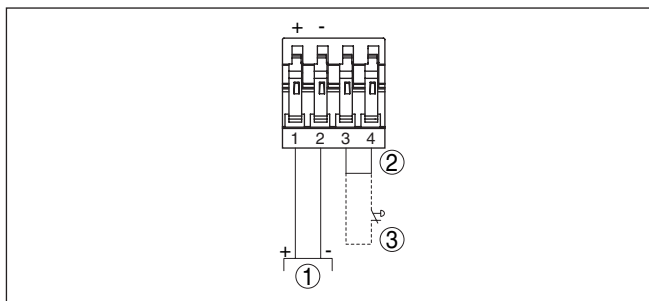
Fig. 10: Wiring plan - External simulation key
