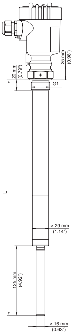
Fig. 34: VEGA VIB 63, threaded version G1 (DIN ISO 228/1)
