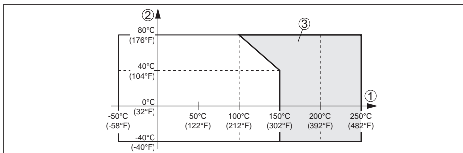
Fig. 31: Ambient temperature - Process temperature
