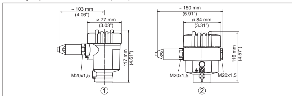
Fig. 33: Housing versions with protection rating IP 66/IP 68 (1 bar)
