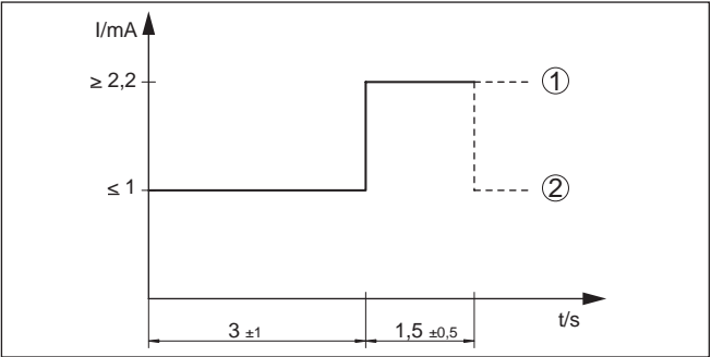
Fig. 22: Flow chart of the function test - Switching function according to the covered and characteristics selection (see function table)
