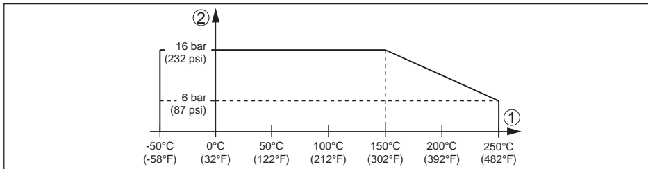
Fig. 30: Process pressure - Process temperature
