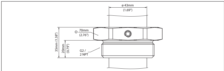
Fig. 2: Lock fitting ARV-WE63.1 unpressurized for VEGAWAVE 63
