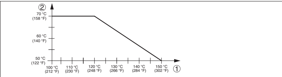
Fig. 17: Ambient temperature - Process temperature
