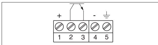
Fig. 5: Transistor output
