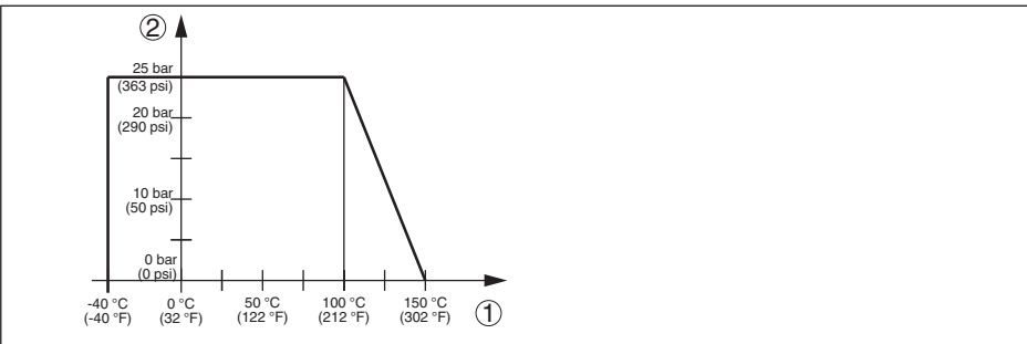
Fig. 18: Process temperature - Process pressure
