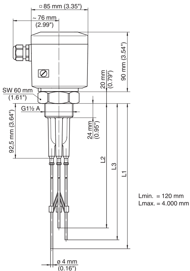
Fig. 23: VEGAKON 66 with three probes
