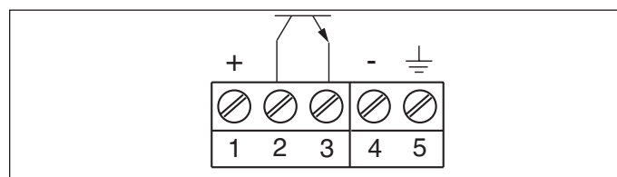
Fig. 9: VEGAKON 61 - transistor output
