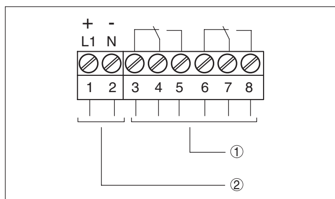
Fig. 8: VEGAKON 66 - electronics with relay output
