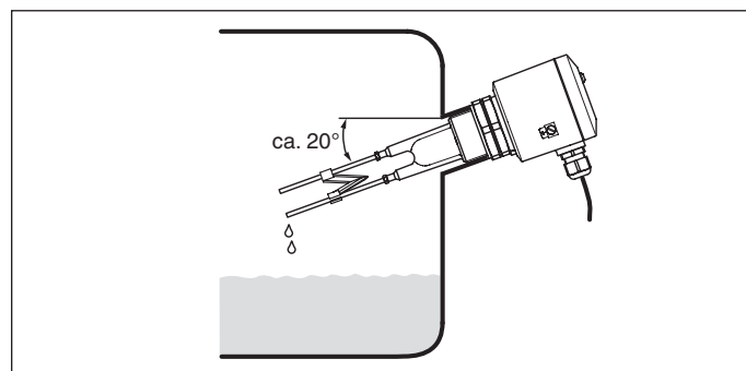
Fig. 6: Horizontal mounting
