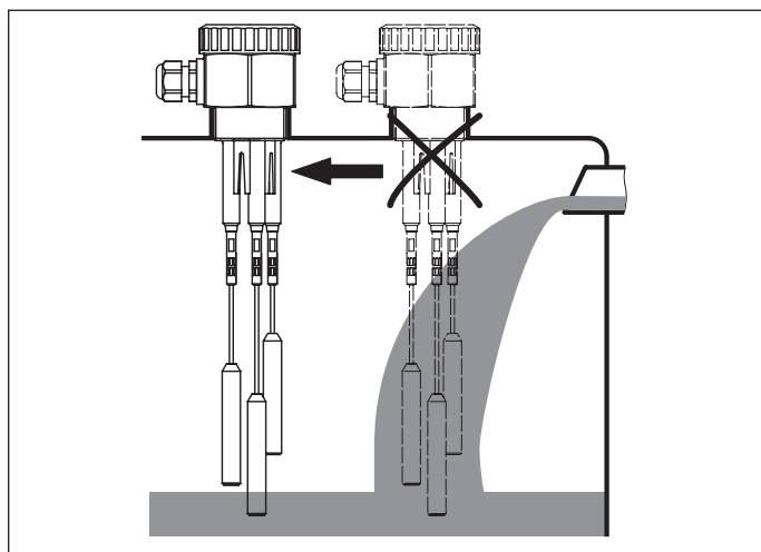
Fig. 12: Instromend medium
