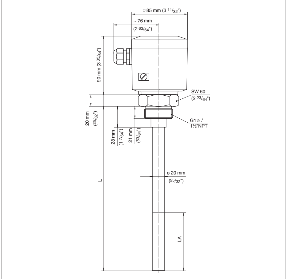
Fig. 10: VEGACAP 27, version filetée G1½ (ISO 228 T1)
