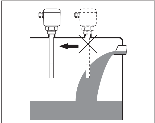
Fig. 4: Instromend medium
