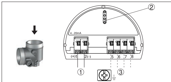
插图. 28: 防爆 (Ex-d-ia) 型双腔式外壳的电子部件腔
