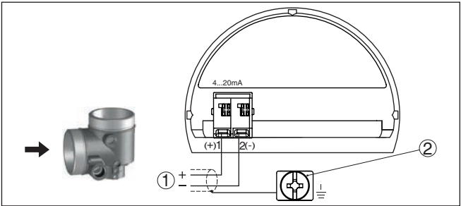
插图. 29: 防爆 (Ex-d-ia) 型双腔式壳体的接线腔
