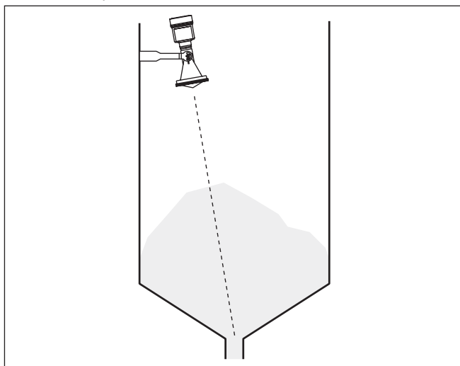
Fig. 13: Montage in open tank
