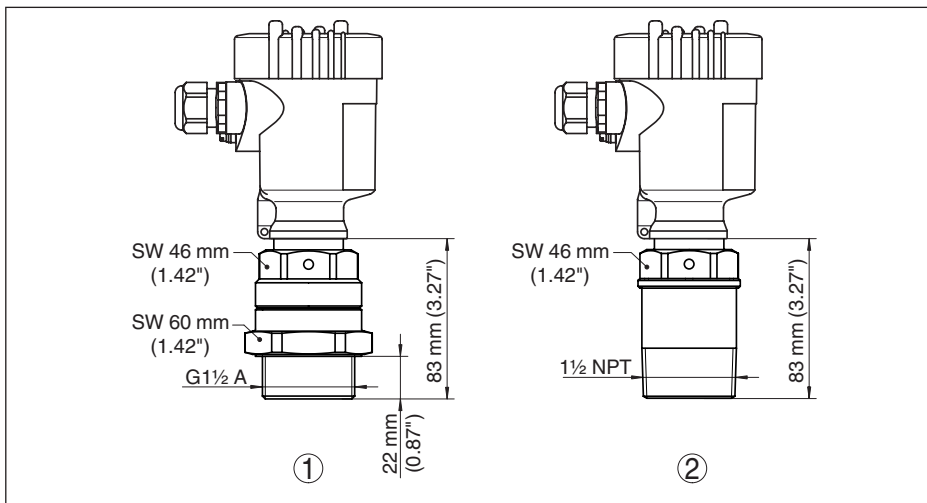
Fig. 9: VEGAMIP 61, internal horn antenna (threaded version)
