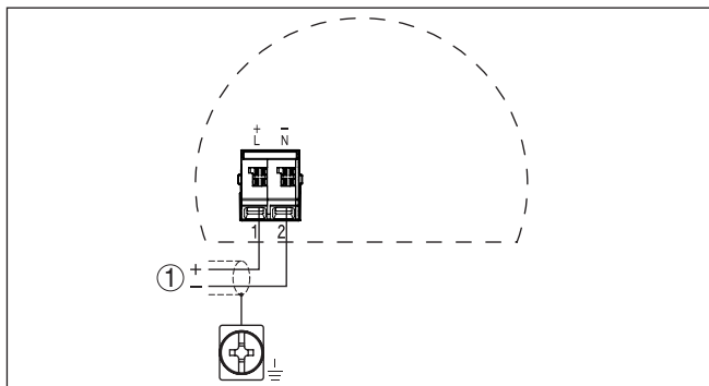
Fig. 7: Wiring plan emitting unit - VEGAMIP 61 (transmitter)
