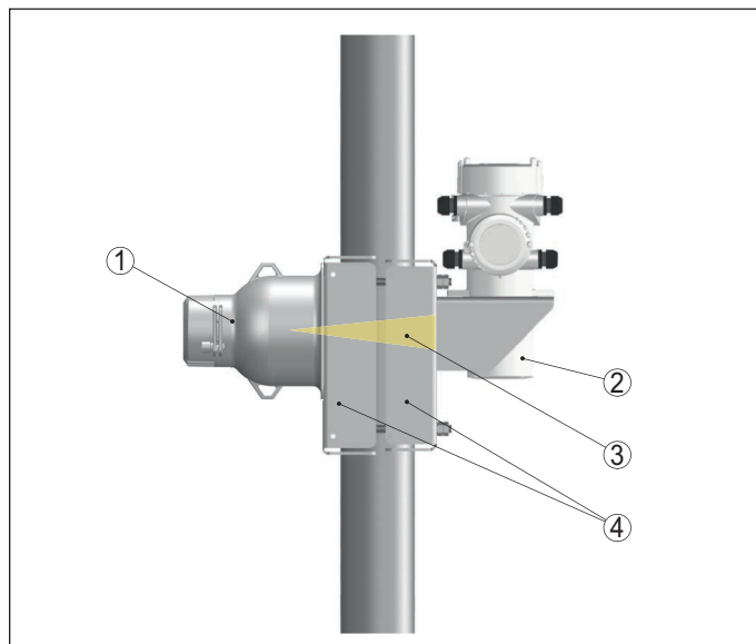
Fig. 6: Measurement arrangement on a pipeline with a diameter of 100 ... 420 mm, detector mounting vertically
