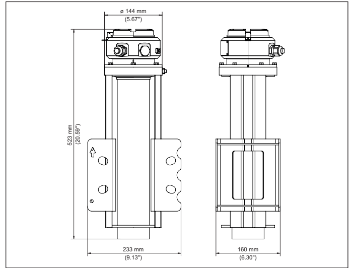
Fig. 37: Gamma modulator for uninterrupted measurement even with X-ray radiation
