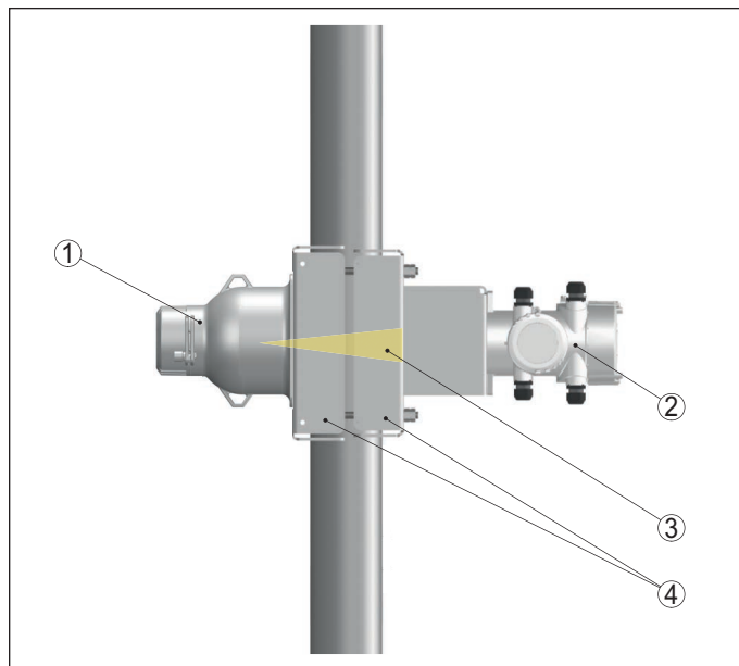
Fig. 7: Measurement setup on a pipeline with a diameter of 100 ... 420 mm, detector mounted horizontally
