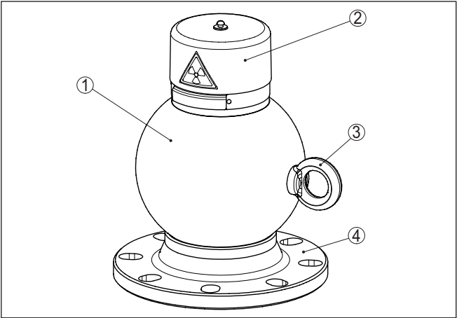
Fig. 9: Conteneur blindé VEGASOURCE 31
