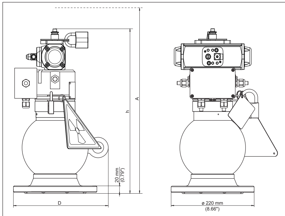
Fig. 51: Conteneur blindé VEGASOURCE 31 - Version K, L
