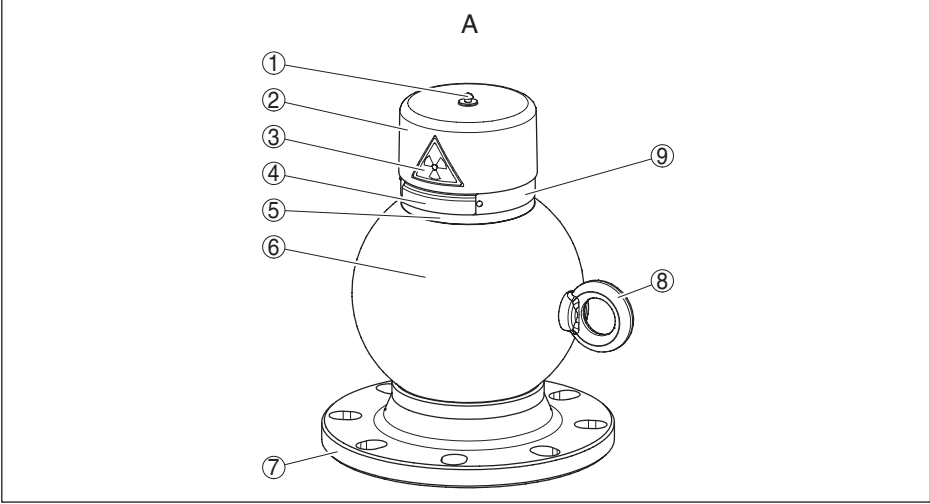
Res. 38: Malzemeler VEGASOURCE 35 - A modeli
