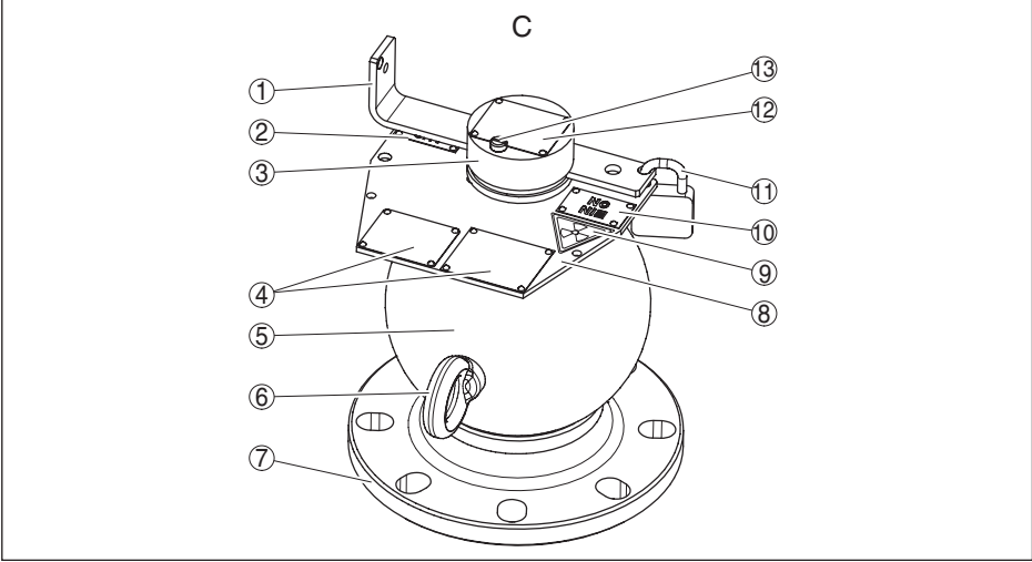
Res. 40: Malzemeler VEGASOURCE 35 - C modeli
