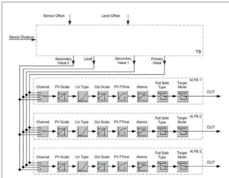
Fig. 54: VEGAPULS SR 68: Block diagram with AI FB 1 ... AI FB 3 OUT values
