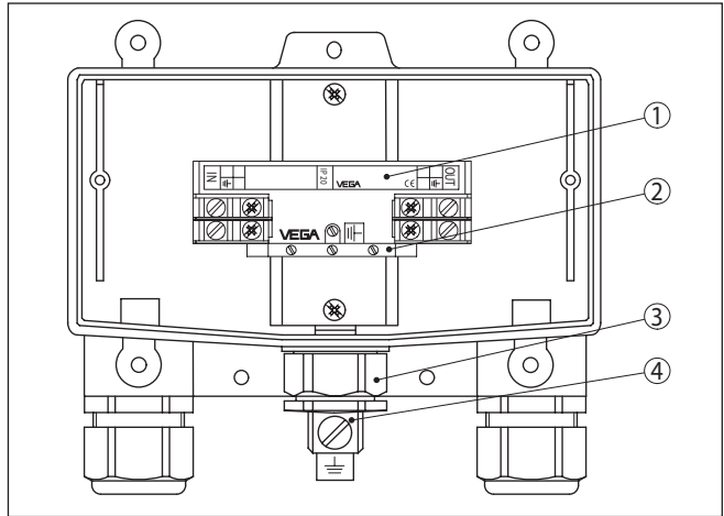
Fig. 6: Mounting in plastic housing
