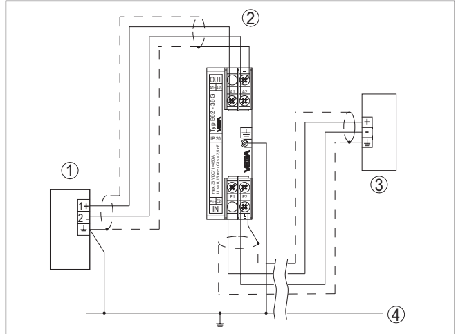
Fig. 8: Wiring plan B62-36G - Sensor protection
