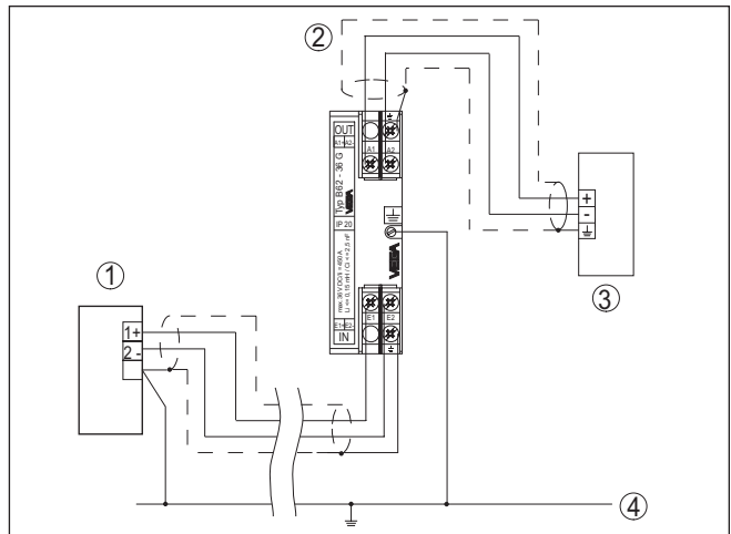
Fig. 9: Wiring plan B62-36G - signal conditioning instrument protection
