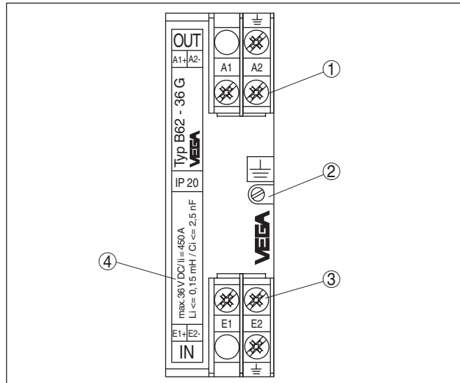
Fig. 1: Configuration of B62-36G
