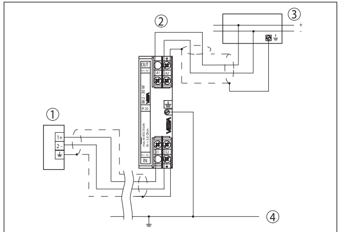
Fig. 9: Wiring plan B62-30W - Protection for bus system
