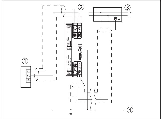
Fig. 8: Wiring plan B62-30W - Sensor protection
