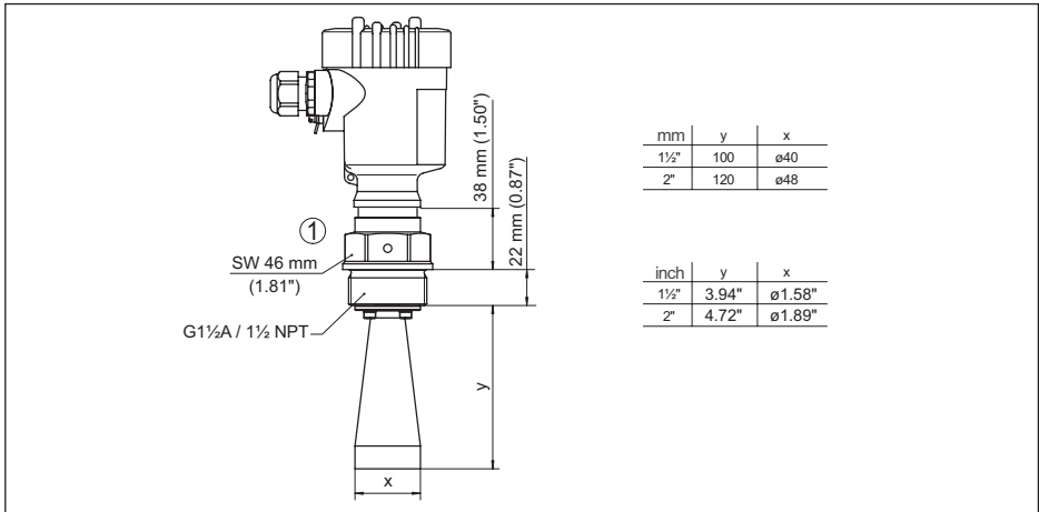
Abb. 32: VEGAMIP 61, Hornantenne/316L
