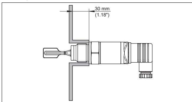
Fig. 6: Aanhechtend product
