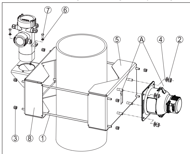
Fig. 6: Mounting bracket with vertically mounted sensor
