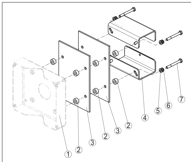
Fig. 7: Mounting of the heat protection plates
