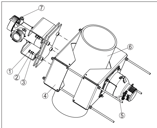
Fig. 10: Mounting bracket with heat protection kit
