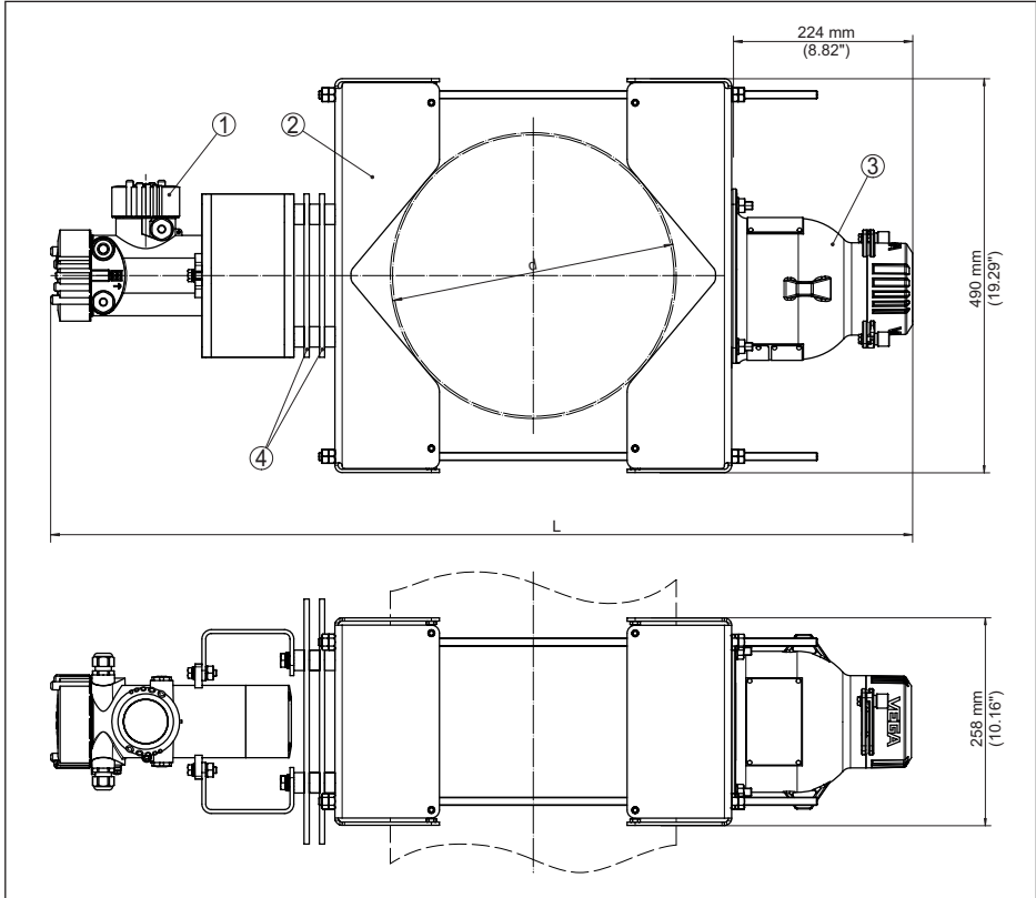
Fig. 15: Mounting bracket with horizontally mounted sensor and heat protection kit (with VEGASOURCE 81, 82)
