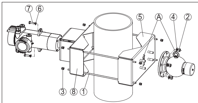
Fig. 5: Mounting bracket with horizontally mounted sensor
