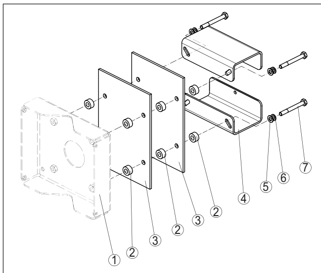
Fig. 11: Mounting of the heat protection plates
