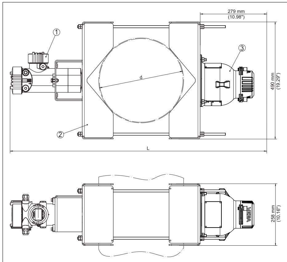
Fig. 14: Mounting bracket with horizontally mounted sensor (with VEGASOURCE 81, 82)
