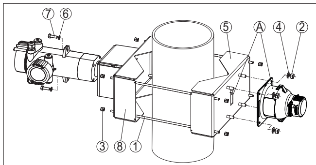
Fig. 8: Mounting bracket with horizontally mounted sensor
