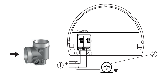
插图. 19: 防爆 (d-ia) 型双腔式外壳的接线腔
