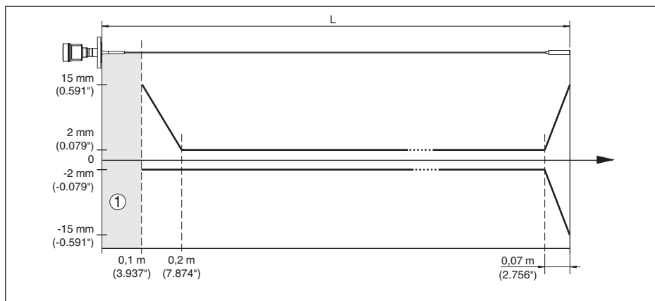
Fig. 34: Meetafwijking VEGAFLEX 83 in kabeluitvoering (bekleed) in product water
