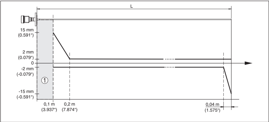
Fig. 29: Meetafwijking VEGAFLEX 83 in staafuitvoering (bekleed) in product water
