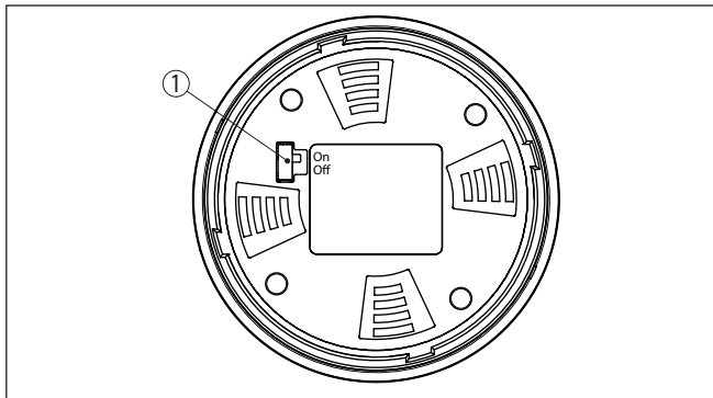
Fig. 20: Bluetooth activeren
