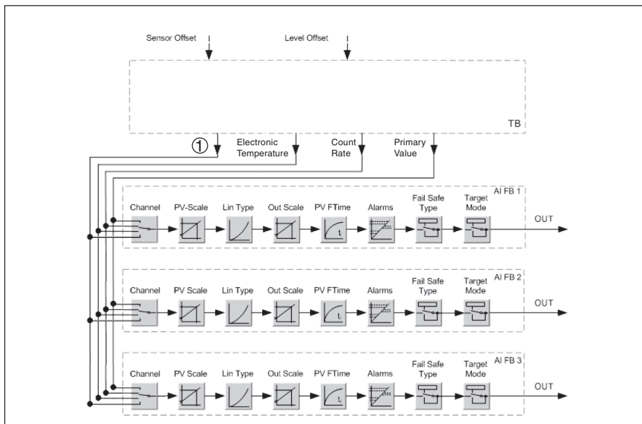
Fig. 27: FIBERTRAC 31: Block diagram with AI FB 1 ... AI FB 3 OUT values
