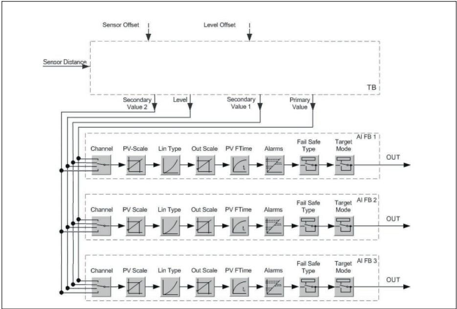
Fig. 43: VEGAFLEX 86: Block diagram with AI FB 1 ... AI FB 3 OUT values
