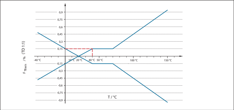
Fig. 51: Determination of the basic temperature error for the above example: F_{\text{TBasis}} = 0.15 \%
