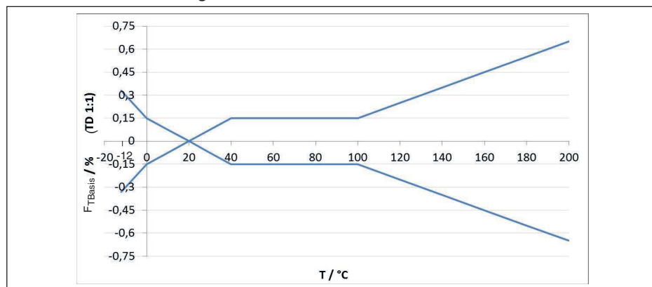
Fig. 44: Basic temperature error F_{TBasis} at TD 1:1
