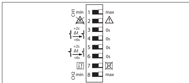
Fig. 2: DIL-schakelaar VEGATOR 122
