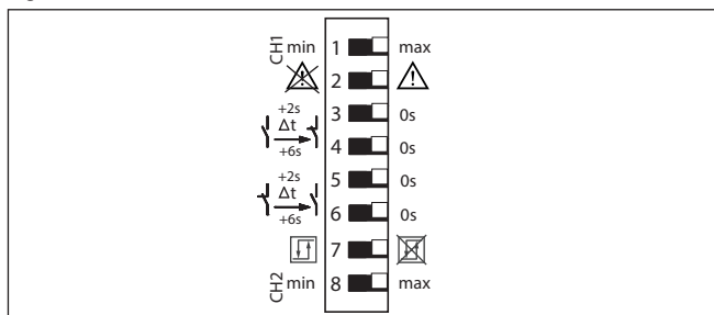
Fig. 3: Interruptor DIL VEGATOR 122
