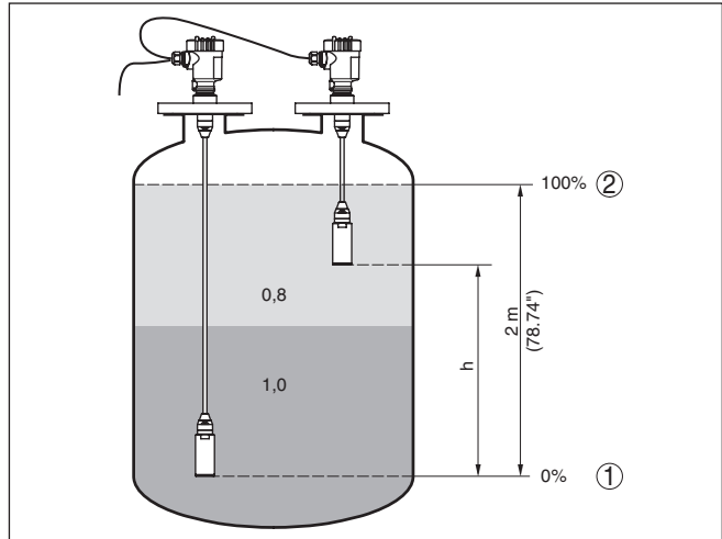
Fig. 5: Parameter adjustment example "Min./max. adjustment, interface measurement"
