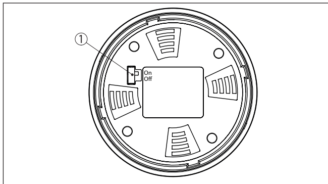
Fig. 11: Bluetooth activeren
