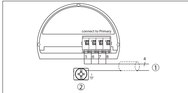
Abb. 4: Anschlussplan VEGABAR 81 Secondary Device
