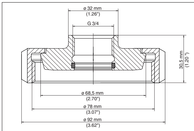
Fig. 57: Dimensions of threaded adapter G \frac{3}{4} (DIN 3852-X) on slotted nut DN 50 (DIN 11851) PN 16
