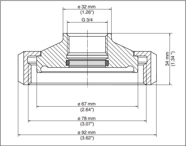
Fig. 45: Dimensions of threaded adapter G \frac{3}{4} (DIN 3852-X) on slotted nut DN 50 (DIN 11864-1) PN 16
