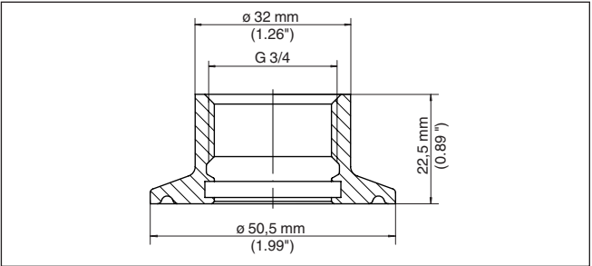
Fig. 53: Dimensions of threaded adapter G¾ (DIN 3852-X) on Clamp 1½" (DIN 32676, ISO 2852) PN 16
