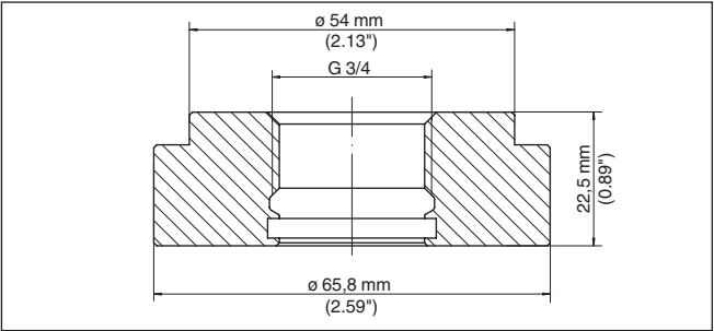
Fig. 47: Dimensions adapter G \frac{3}{4} (DIN 3852-X) on DRD
