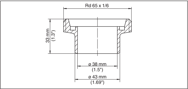
Fig. 11: Dimensions of welded socket, slotted nut DN 40 (DIN 11851)
