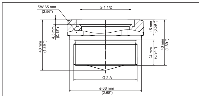
Fig. 35: Dimensions of threaded adapter G1½ (DIN 3852-X) on thread G2 (DIN 3852-X)
