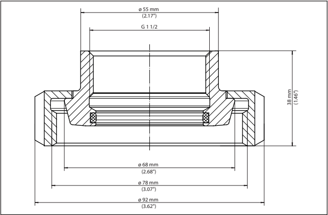
Fig. 43: Dimensions of threaded adapter G1½ (DIN 3852-X) on slotted nut DN 50 (DIN 11851) PN 16
