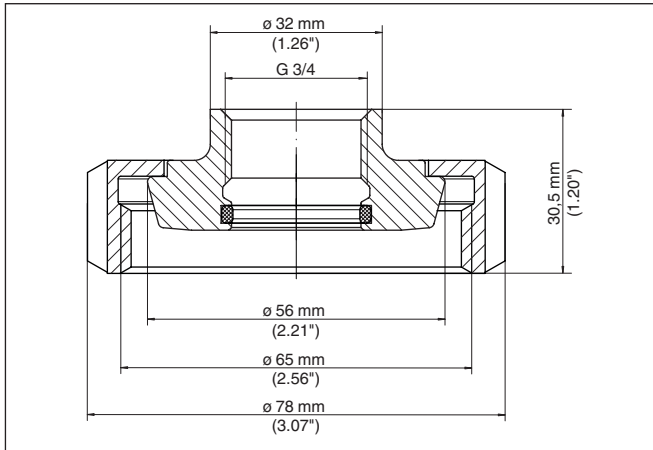
Fig. 41: Dimensions of threaded adapter G \frac{3}{4} (DIN 3852-X) on slotted nut DN 40 (DIN 11851) PN 16
