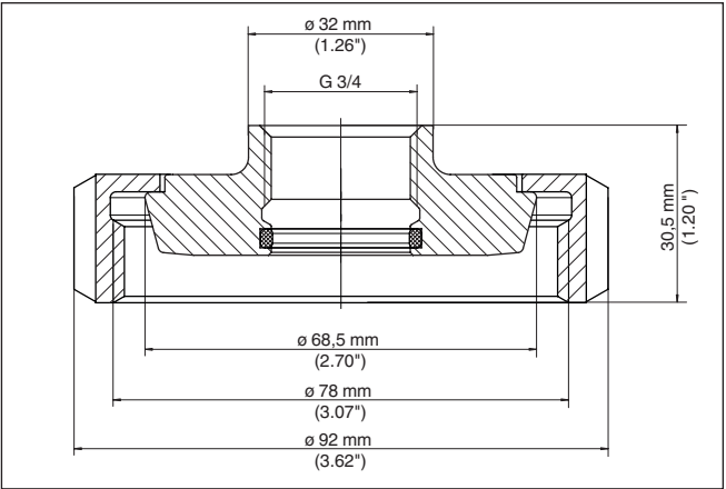
Fig. 56: Dimensions of threaded adapter G¾ (DIN 3852-X) on slotted nut DN 50 (DIN 11851) PN 25
