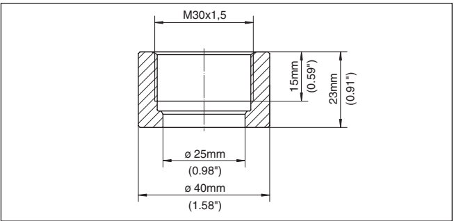
Fig. 24: Dimensions of welded socket, M30 x 1.5 - VEGABAR 82
