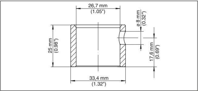
Fig. 27: Dimensions of welded socket, PMC 1" VEGABAR 82
