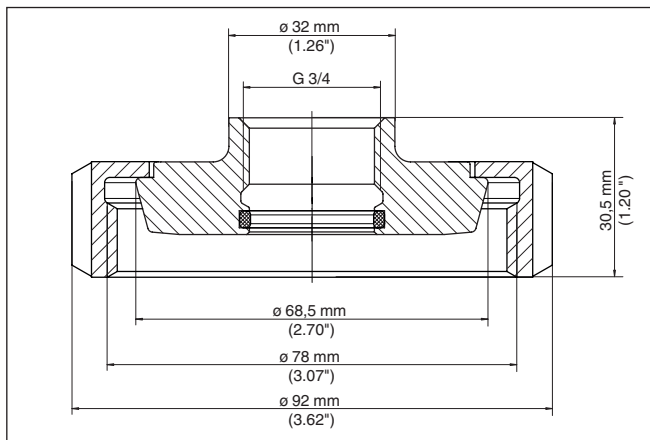
Fig. 42: Dimensions of threaded adapter G \frac{3}{4} (DIN 3852-X) on slotted nut DN 50 (DIN 11851) PN 16
