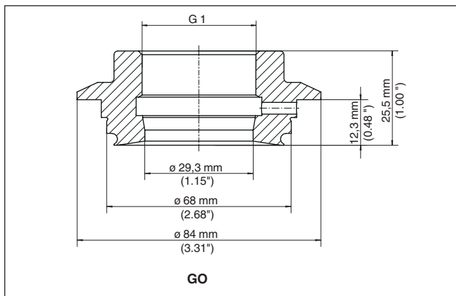
Fig. 52: Dimensions of threaded adapter G1 (DIN 3852-X) on Varivent Form N 50-40
