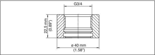
Fig. 21: Dimensions of welded socket, G3/4 (DIN 3852-X) - VEGABAR 82
