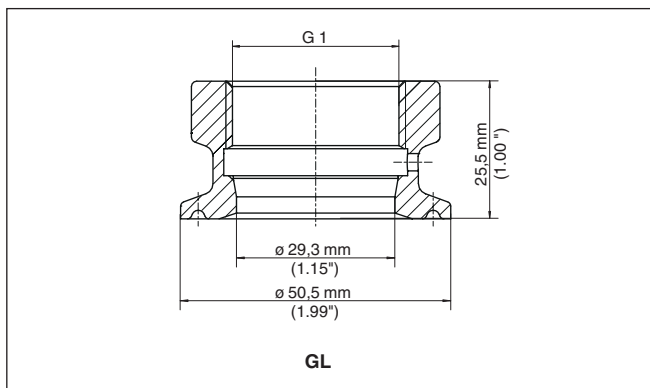
Fig. 49: Dimensions of threaded adapter G1 (DIN 3852-X) on Clamp 1½" (DIN 32676, ISO 2852) PN 16
