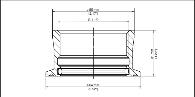
Fig. 58: Dimensions of threaded adapter G1½ (DIN 3852-X) on Clamp 2" (DIN 32676, ISO 2852) PN 16
