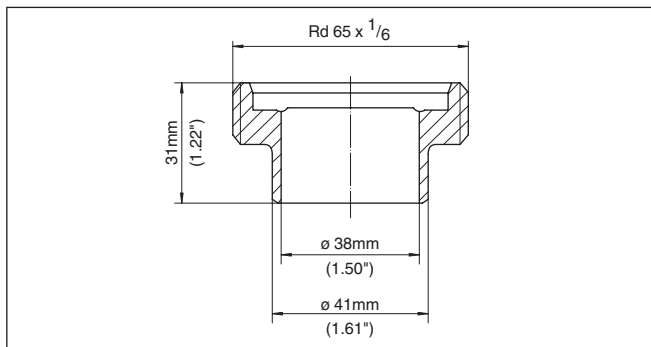
Fig. 13: Dimensions of welded socket, slotted nut DN 40 (DIN 11864-1)
