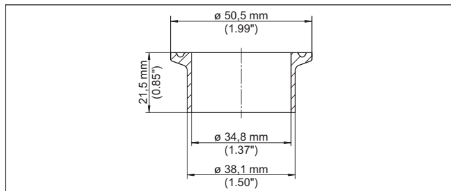
Fig. 9: Dimensions of welded socket, Clamp 1½" (DIN 32676, ISO 2852) PN 16
