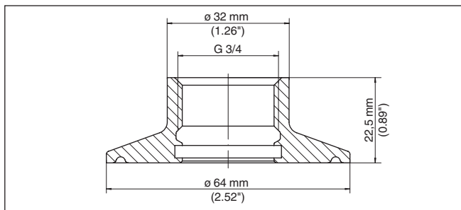
Fig. 54: Dimensions of threaded adapter G1½ (DIN 3852-X) on Clamp 2" (DIN 32676, ISO 2852) PN 16
