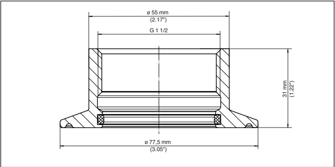
Fig. 59: Dimensions of threaded adapter G1½ (DIN 3852-X) on Clamp 2½" (DIN 32676, ISO 2852) PN 16
