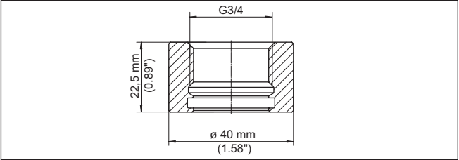
Fig. 7: Dimensions of welded socket, thread G \frac{3}{4} (ISO 228-1) - Hygienic design
