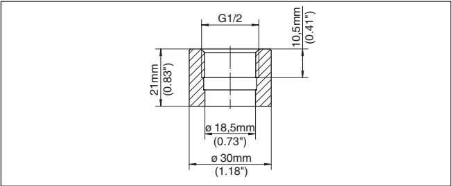
Fig. 20: Dimensions welded socket G1/2 (ISO 228-1), front-flush - VEGABAR 82
