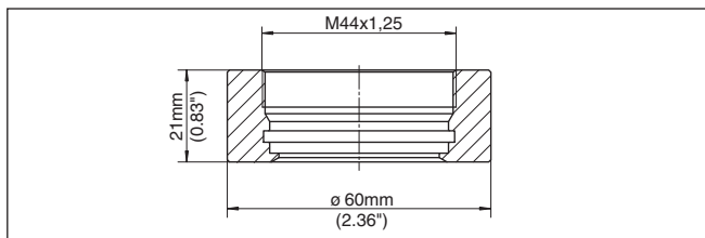
Fig. 25: Dimensions of welded socket, M44 x 1.25 - VEGABAR 82, 83
