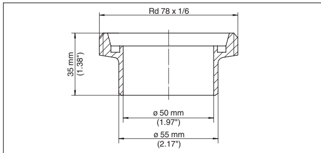
Fig. 12: Dimensions of welded socket, slotted nut DN 50 (DIN 11851)
