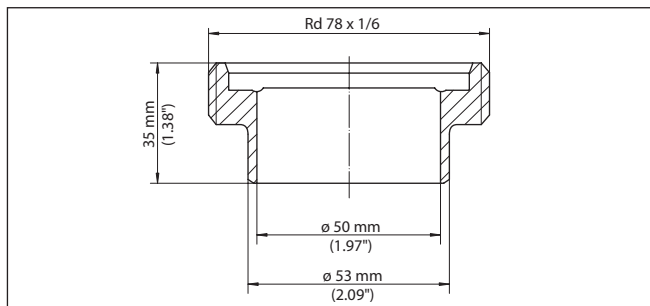
Fig. 14: Dimensions of welded socket, slotted nut DN 50 (DIN 11864-1)
