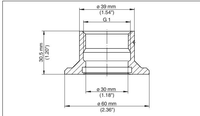
Fig. 33: Dimensions of welded socket, G1 (DIN 3852-X) - suitable for foodstuffs
