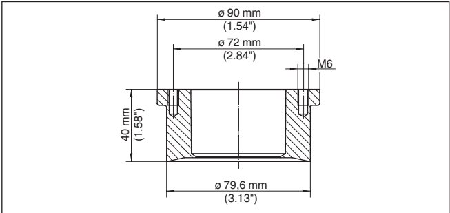
Fig. 16: Dimensions of welded socket, hygienic fitting DN 32 with tension flange
