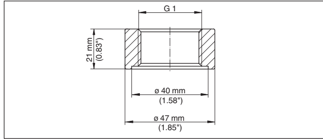
Fig. 32: Dimensions of welded socket, G1 (DIN 3852-X)
