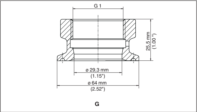
Fig. 50: Dimensions of threaded adapter G1 (DIN 3852-X) on Clamp 2" (DIN 32676, ISO 2852) PN 16
