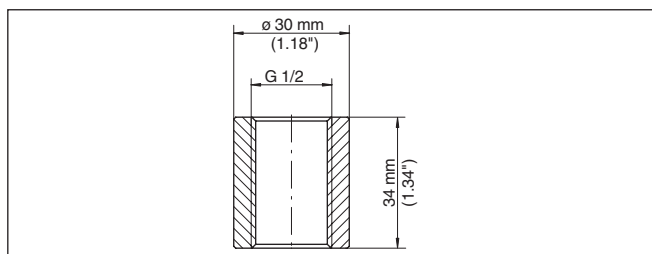
Fig. 19: Dimensions of welded socket, thread G \frac{1}{2} (EN 837) - manometer connection - VEGABAR 81, 82, 83
