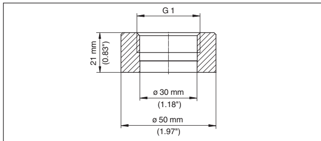
Fig. 22: Dimensions of welded socket, G1 (ISO 228-1) - VEGABAR 82, 83
