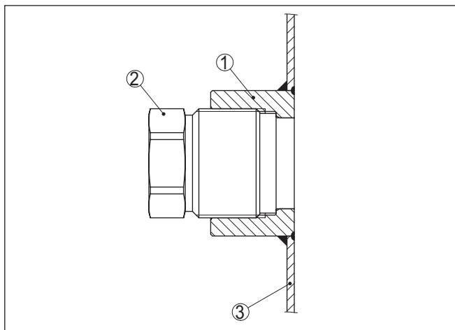
Fig. 62: Welding dummy
