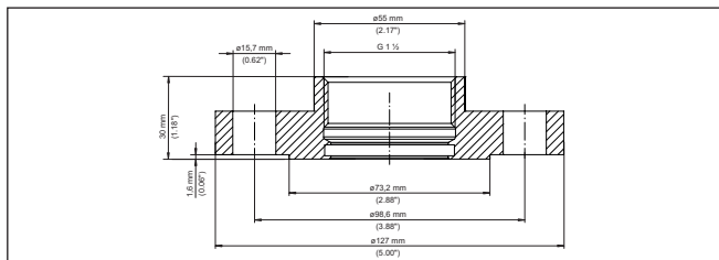
Fig. 37: Dimensions of threaded adapter G1½ (DIN 3852-X) on flange 1½" (ASME B16.5, RF) 150 lb
