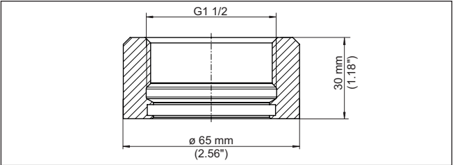
Fig. 8: Dimensions of welded socket, thread G1 \frac{1}{2} (ISO 228-1) - Hygienic design
