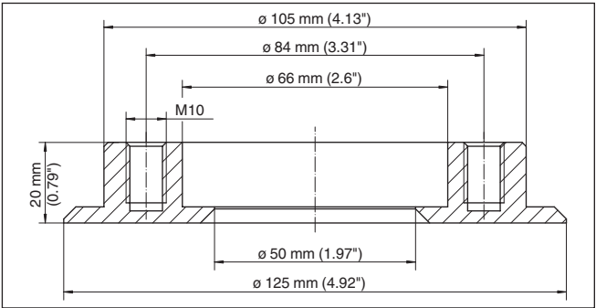
Fig. 17: Dimensions of welded socket, DRD
