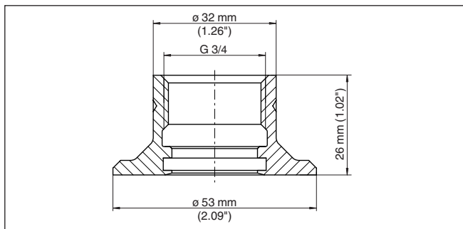
Fig. 28: Dimensions of welded socket, G \frac{3}{4} (DIN 3852-X)
