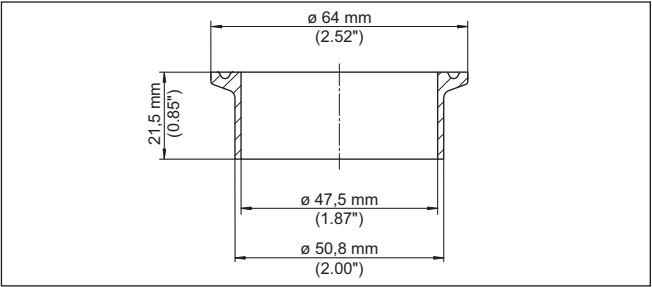
Fig. 10: Dimensions of welded socket, Clamp 2" (DIN 32676, ISO 2852) PN 16
