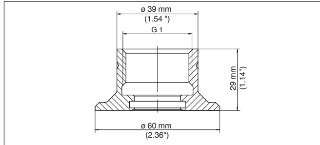
Fig. 29: Dimensions of welded socket, G1 (DIN 3852-X)
