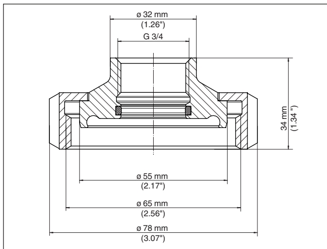
Fig. 44: Dimensions of threaded adapter G \frac{3}{4} (DIN 3852-X) on slotted nut DN 40 (DIN 11864-1) PN 16
