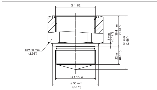
Fig. 34: Dimensions of threaded adapter G1½ (DIN 3852-X) on thread G1½, G2 (DIN 3852-X)
