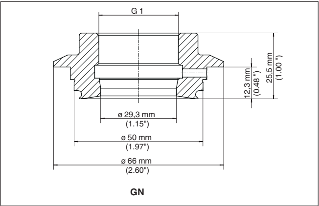
Fig. 51: Dimensions of threaded adapter G1 (DIN 3852-X) on Varivent Form F 25
