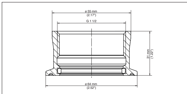
Fig. 40: Dimensions of threaded adapter G1 \frac{1}{2} (DIN 3852-X) on Clamp 2" (DIN 32676, ISO 2852) PN 16
