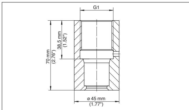
Fig. 26: Dimensions welded socket G1 suitable for PASVE (for the two previously listed versions) - VEGABAR 82
