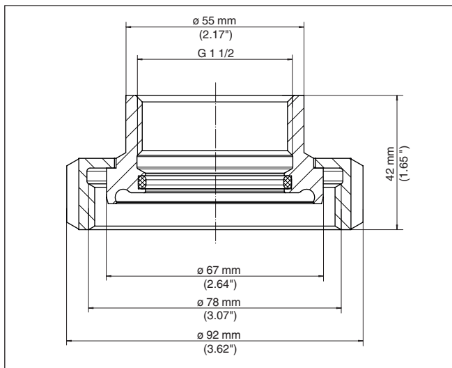
Fig. 46: Dimensions of threaded adapter G1½ (DIN 3852-X) on slotted nut DN 50 (DIN 11864-1) PN 16
