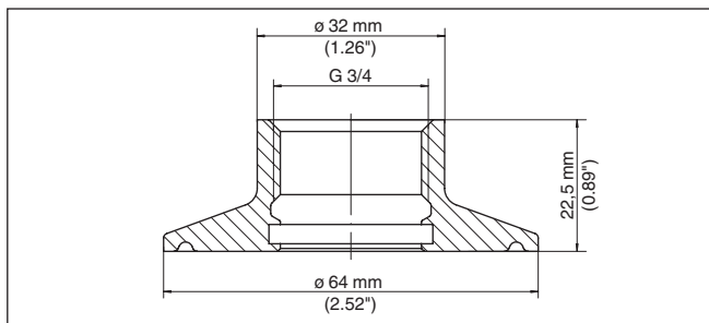
Fig. 39: Dimensions of threaded adapter G \frac{3}{4} (DIN 3852-X) on Clamp 2" (DIN 32676, ISO 2852) PN 16
