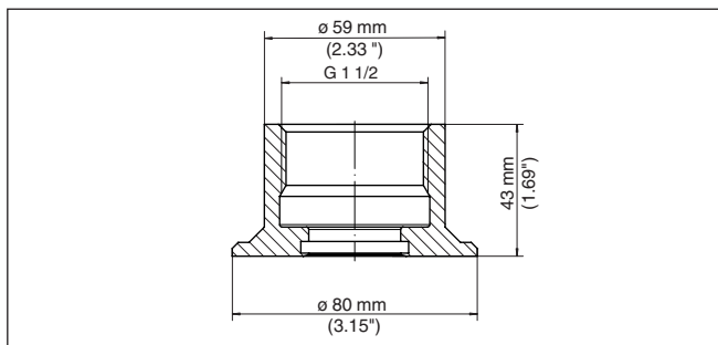
Fig. 31: Dimensions of welded socket, G1½ (DIN 3852-A)
