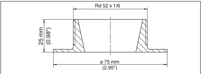
Fig. 18: Dimensions of welded socket, conus connection DN 25
