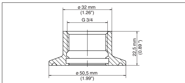
Fig. 38: Dimensions of threaded adapter G \frac{3}{4} (DIN 3852-X) on Clamp 1 \frac{1}{2} " (DIN 32676, ISO 2852) PN 16
