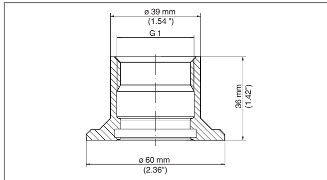
Fig. 30: Dimensions of welded socket, G1 (DIN 3852-A)
