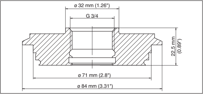
Fig. 48: Dimensions adapter G \frac{3}{4} (DIN 3852-X) on Tuchenhagen DN 32
