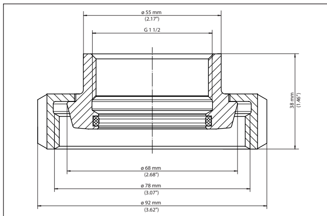
Fig. 60: Dimensions of threaded adapter G1½ (DIN 3852-X) on slotted nut DN 50 (DIN 11851) PN 16
