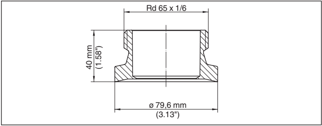
Fig. 15: Dimensions of welded socket, hygienic fitting F40 with compression nut
