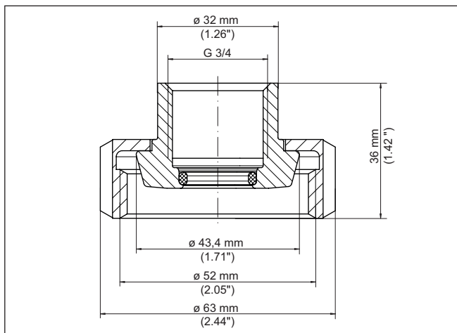
Fig. 55: Dimensions of threaded adapter G¾ (DIN 3852-X) on slotted nut DN 25 (DIN 11851) PN 25
